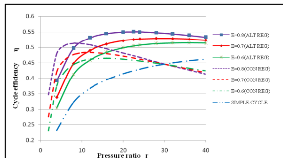
Fig: 6. Effect of Pressure Ratio on Efficiency with Effectiveness [T1=300 K, TIT=1500 0C]
