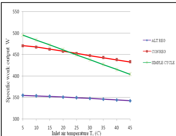
Fig 15: Effect of the Inlet Air Temperature on Specific Work Output [TIT = 1500 0C, r = ropt]
