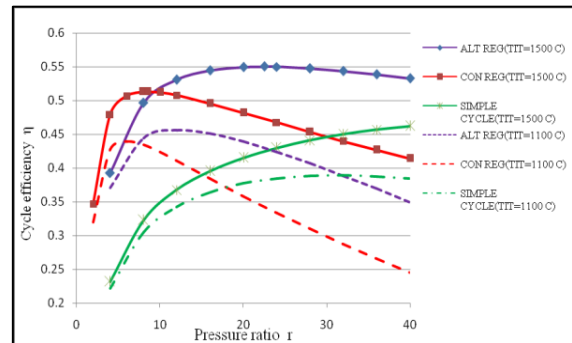
Fig: 6. Effect of Pressure Ratio on Efficiency with Effectiveness [T1=300 K, TIT=1500 0C]
