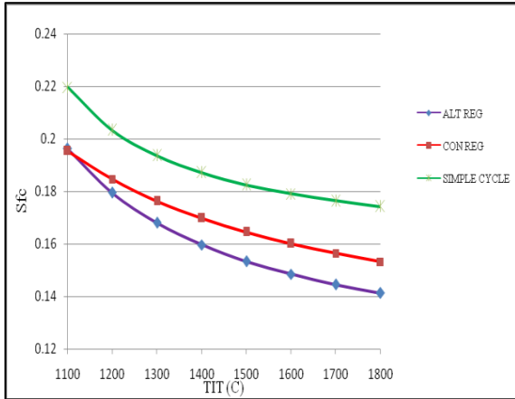
Fig 14: Effect of the Inlet Air Temperature on Efficiency [TIT = 1500 0C, r = ropt]
