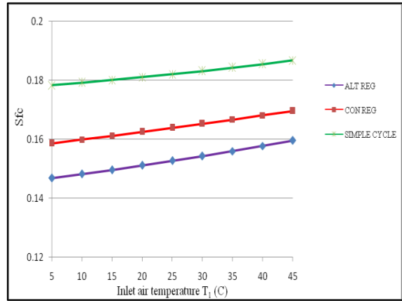
Fig 16: Effect of the Inlet Air Temperature on Specific Fuel Consumption [TIT = 1500 0C, r = ropt]
